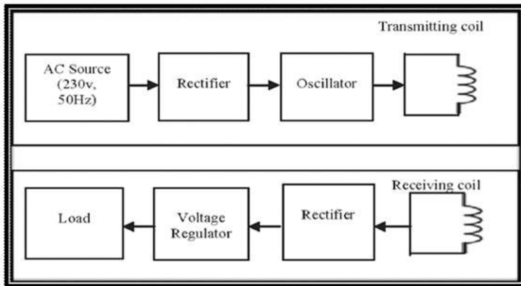
Figure 1: Block Diagram of Wireless Power Transfer System
