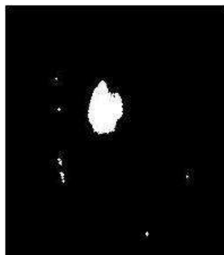
Figure 6: Thresholding Segmentation
