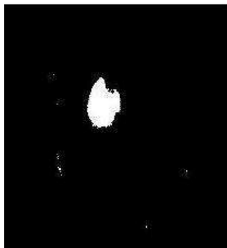
Figure 5: FCM Segmentation
