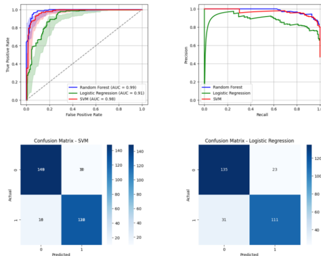
Figure 4: Model Performance Comparison Visualization
